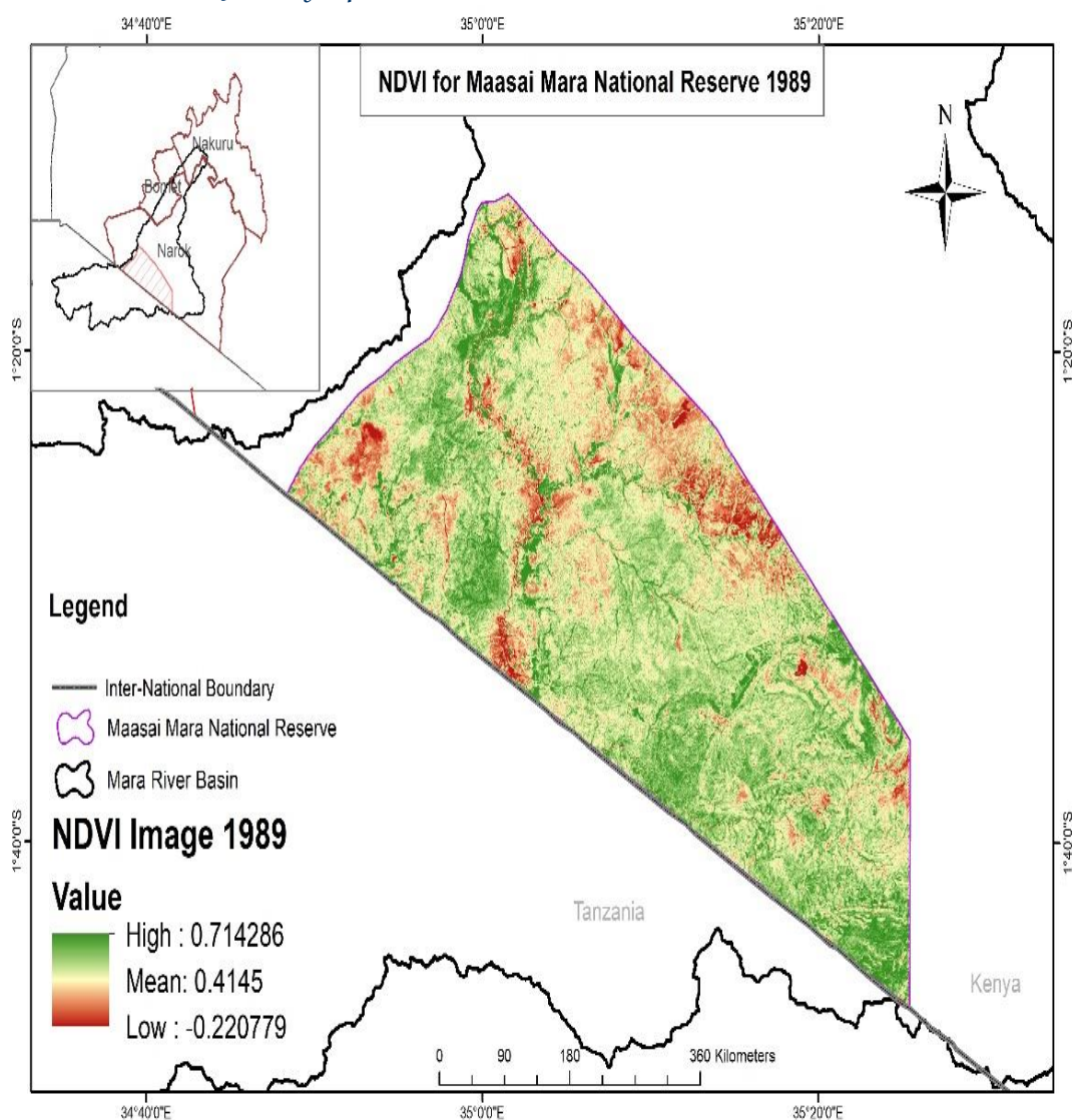
Figure 9: NDVI in 1989
